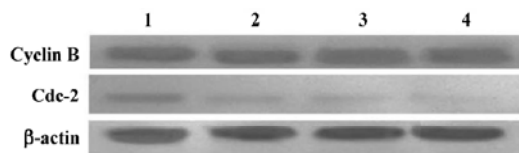
Figure 3. AZ4 alters the expression of cell cycle proteins, cyclin B and Cdc-2. The expression of cyclin B and Cdc-2 were assessed by immunoblotting. The H460 cells treated with various concentrations of AZ4 (lanes 1–4: 0, 0.25, 0.5, and 2 μmol/L, respectively) for 24 h, and cell lysate was prepared for analysis. The immunoblots shown have been equilibrated for protein loading. The data shown were representative of 3 separate experiments.
